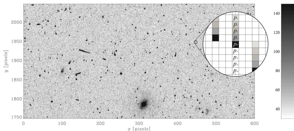
Figure 1: A typical, raw HST ACS / WFC image, in units of electrons. This 30'' \times 15'' (600 \times 300 pixels) region contains warm pixels, with an example warm pixel towards the right zoomed in on. This reveals CTI trailing behind (above) the warm pixel, which PyAutoCTI fits to calibrate CTI. This figure is taken from (Massey et al., 2010) and has been used with the author's permission.
